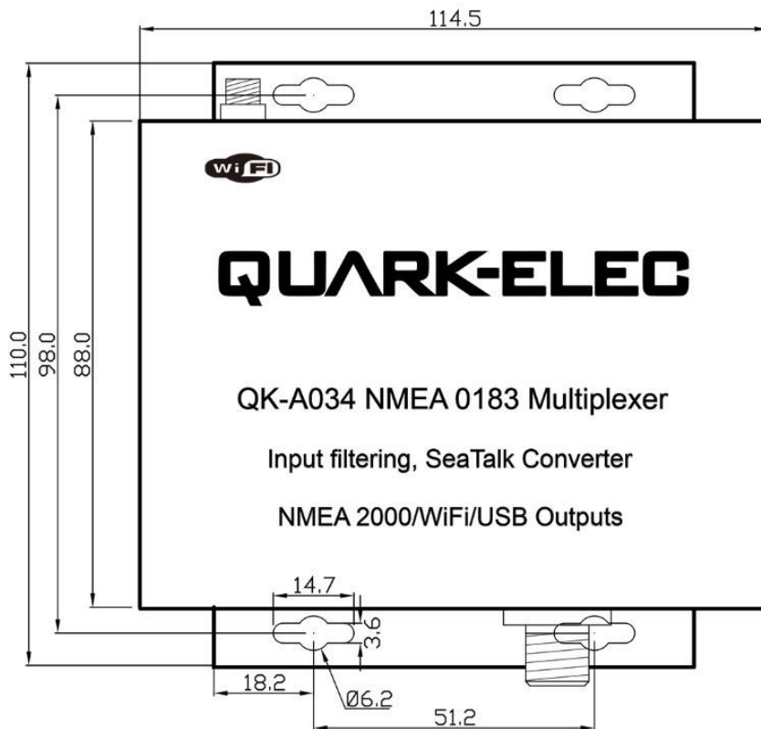
Figure 1:Dimensions
